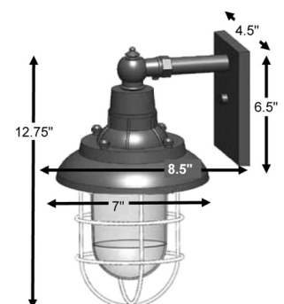
600.10.03-WW (PB Finish)
