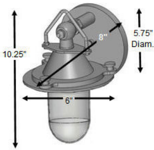
700.10.03-WG (SN Finish)
