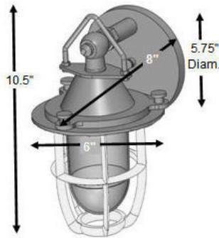
700.10.03-WC (SN Finish)
