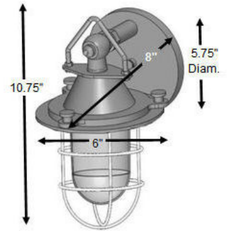
700.10.03-WW (SN Finish)
